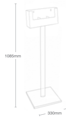
AS3110 Luxury floor stand - 2 x 1/3rd A4 pockets - side by side Opening dimensions: 110 x 32mm Pockets: Crystal Clear Polystyrene
